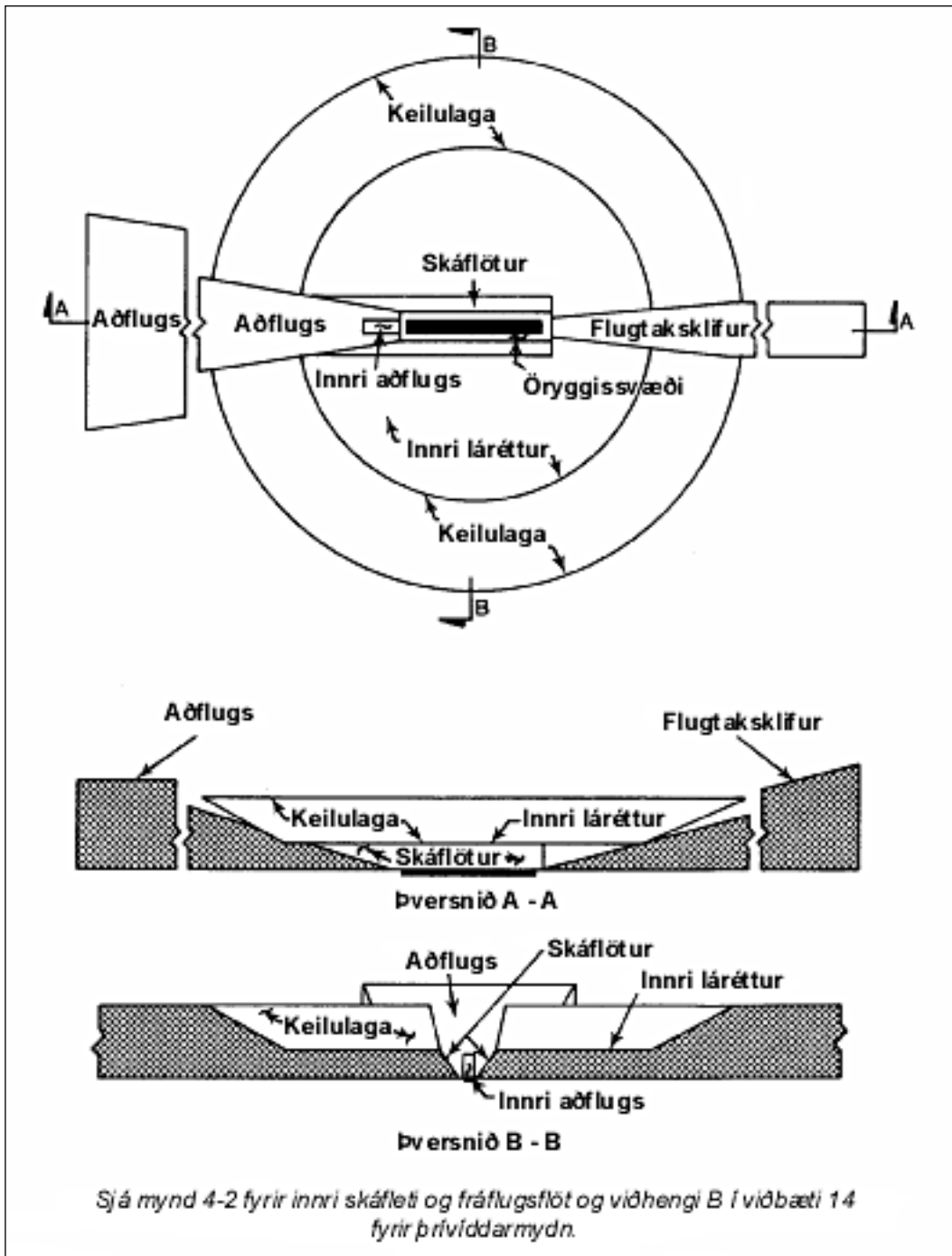
Mynd 4-1. Hindranafletir (Obstacle limitation surfaces).
