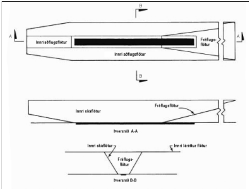
Mynd 4-2. Innri aðflugshindranaflötur, innri skáhindranaflötur og fráflugshindranaflötur (Inner approach, inner transitional and balked landing obstacle limitation surfaces).
