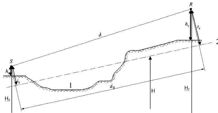
Equivalent heights in relation to the ground
