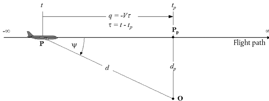
Geometry between flight path and observer location O
